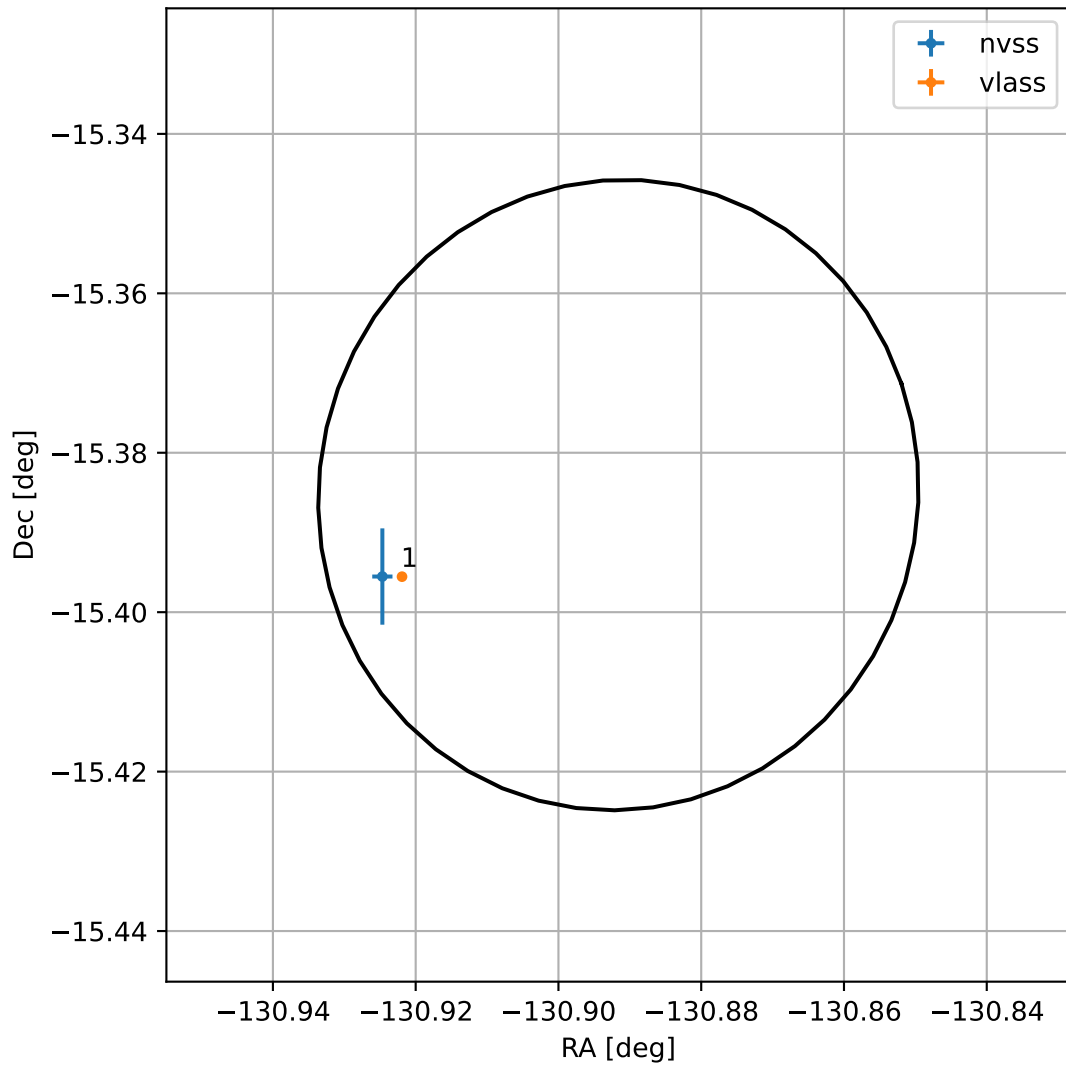
4FGL J1516.4-1523
