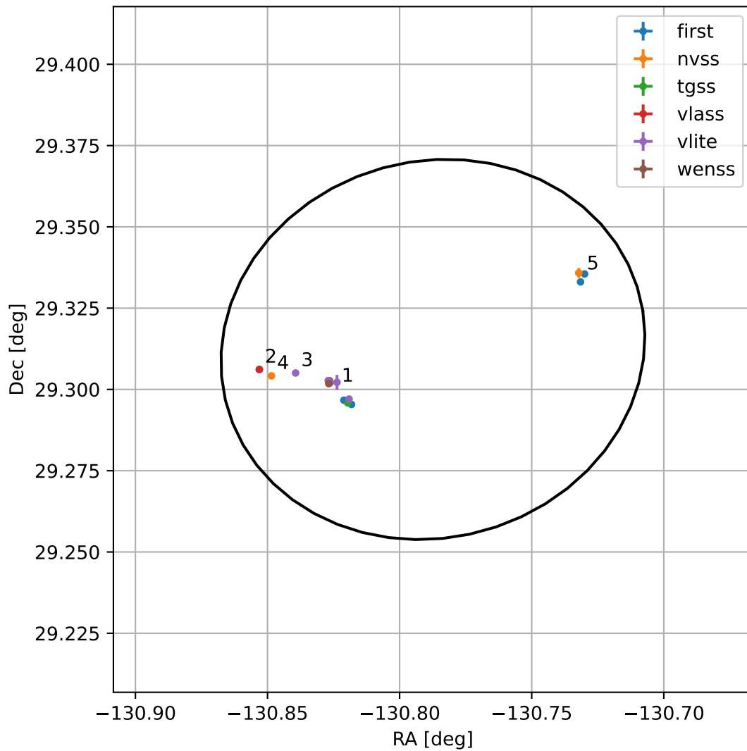
4FGL J1516.8+2918
