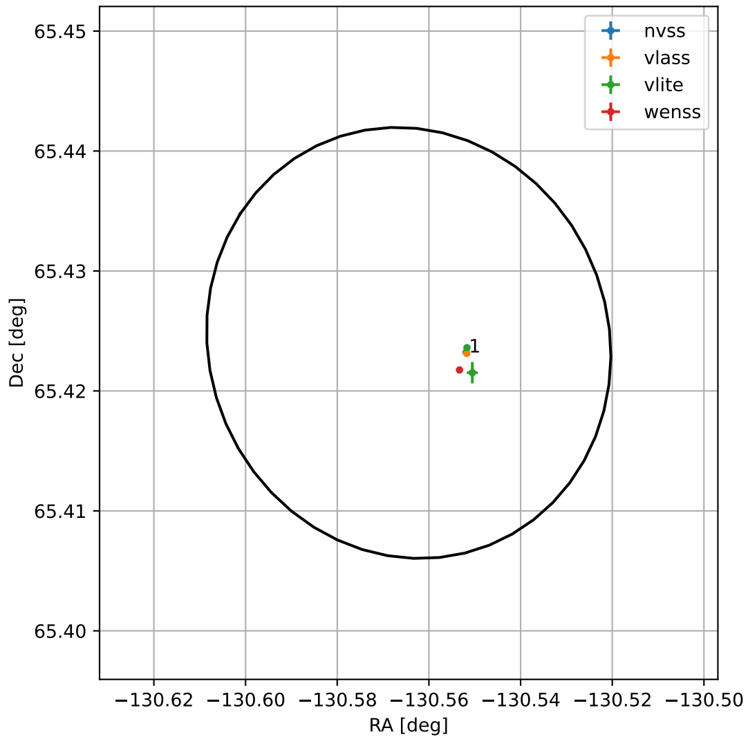
4FGL J1517.7+6525
