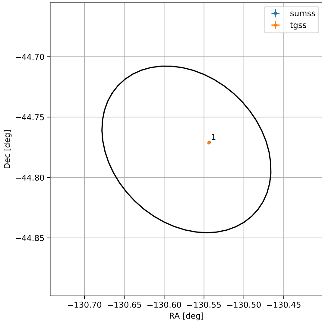
4FGL J1517.7-4446
