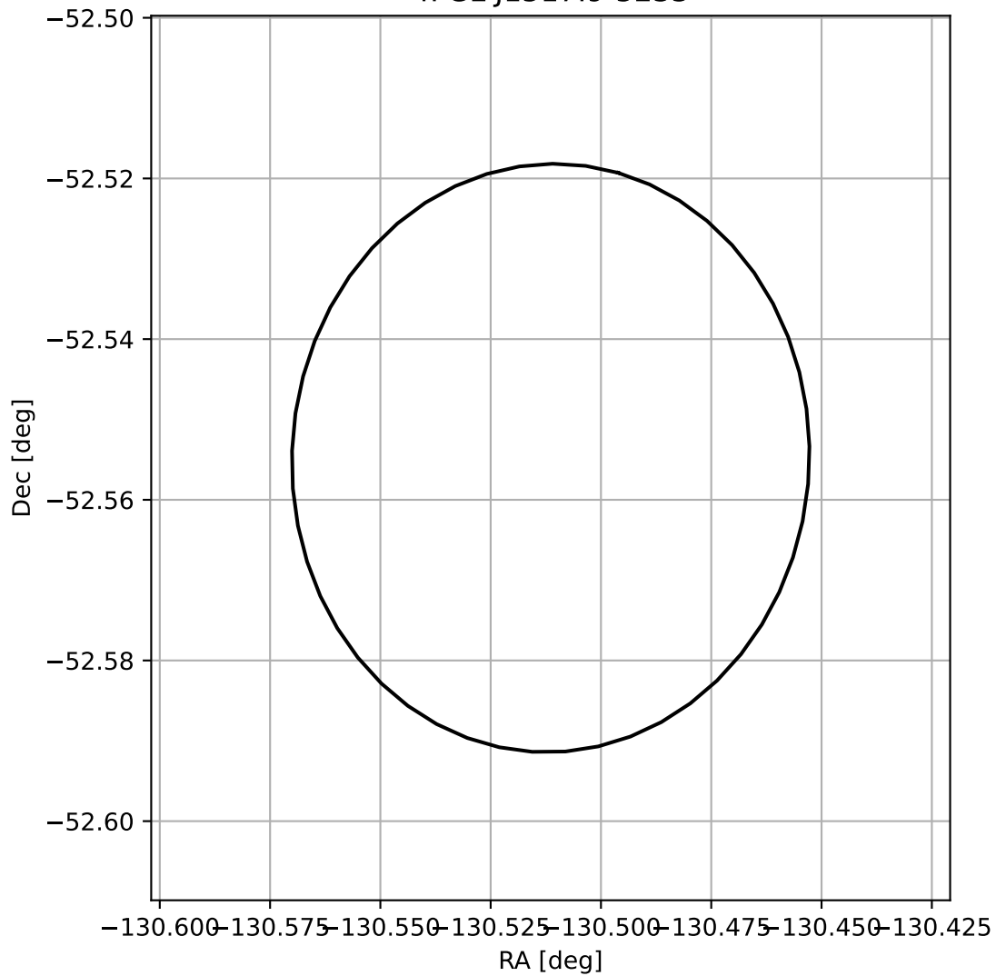
4FGL J1517.9-5233
