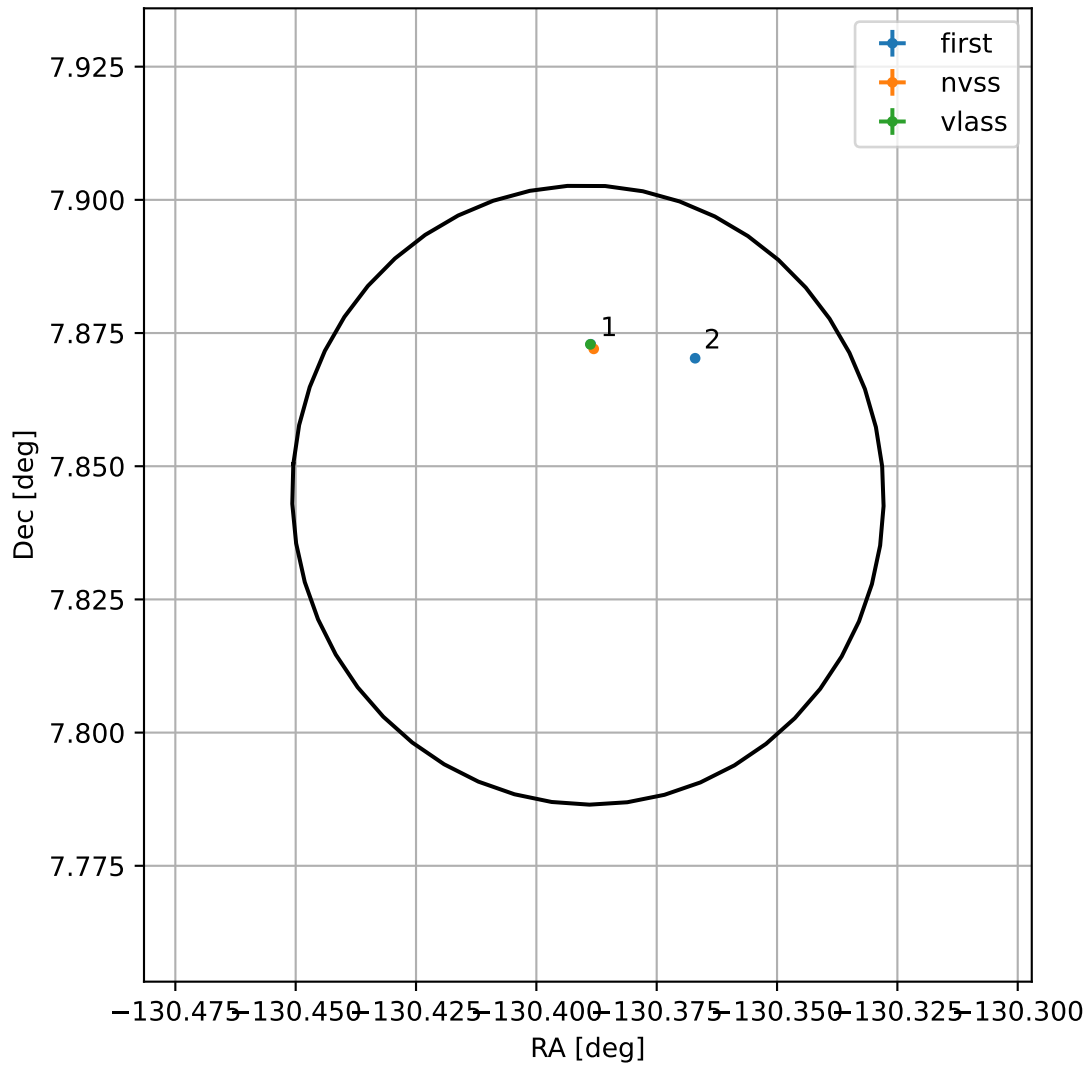
4FGL J1518.4+0750
