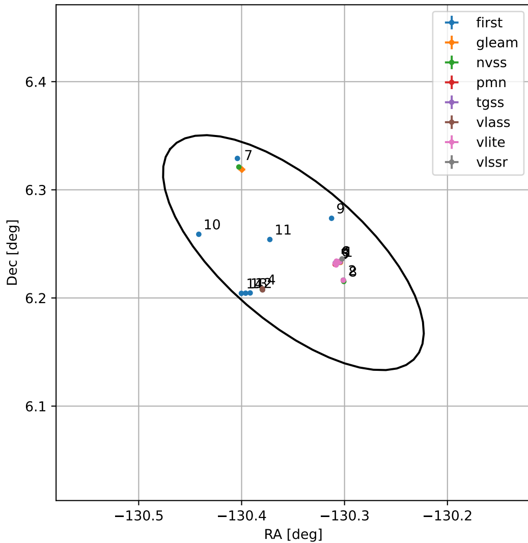
4FGL J1518.6+0614
