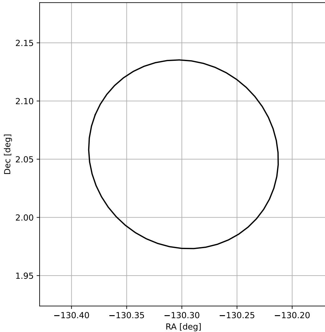
4FGL J1518.8+0203
