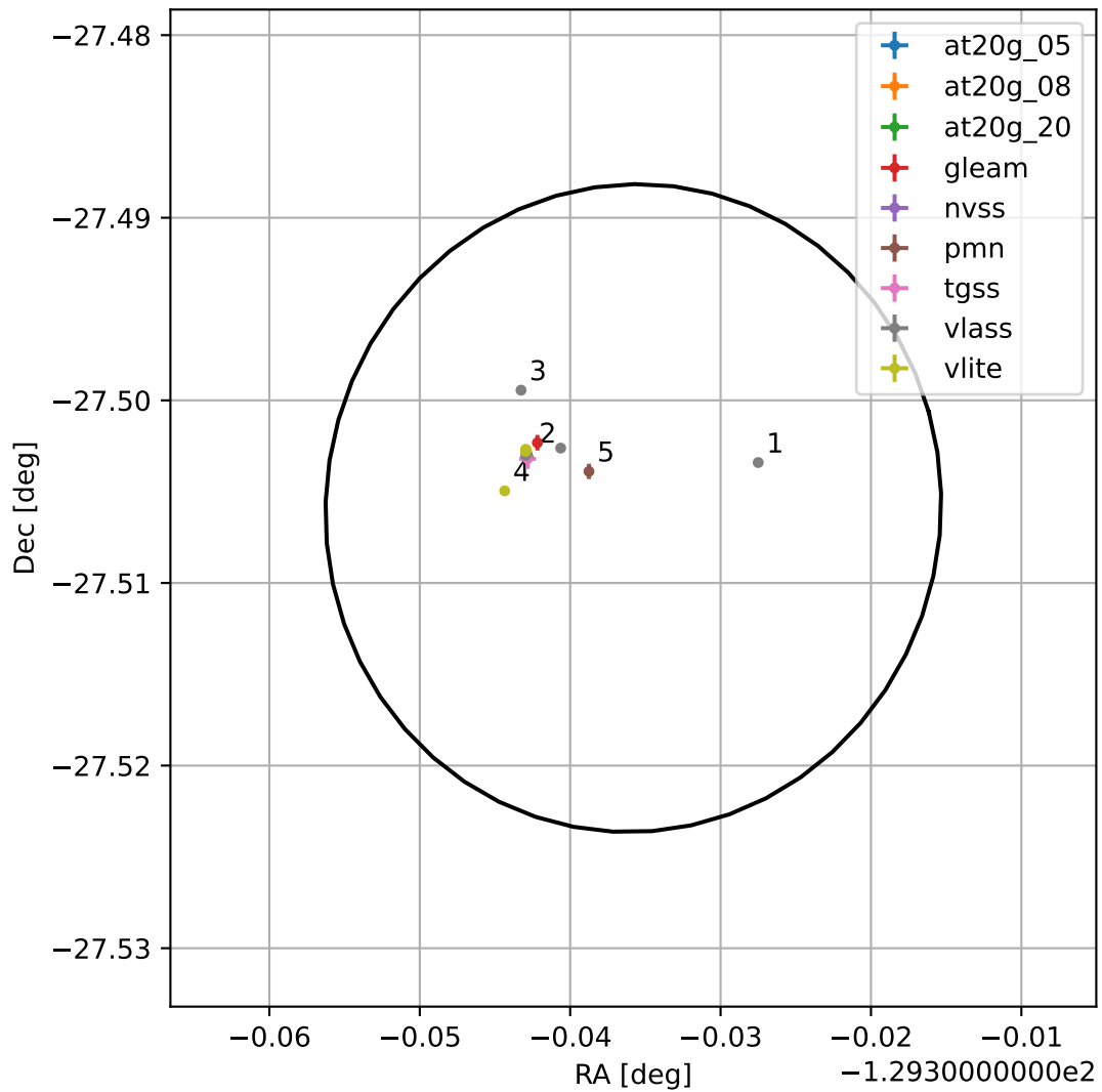
4FGL J1522.6-2730
