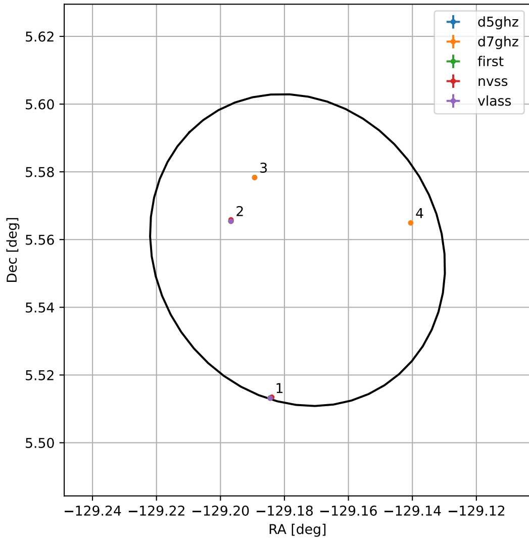
4FGL J1523.2+0533
