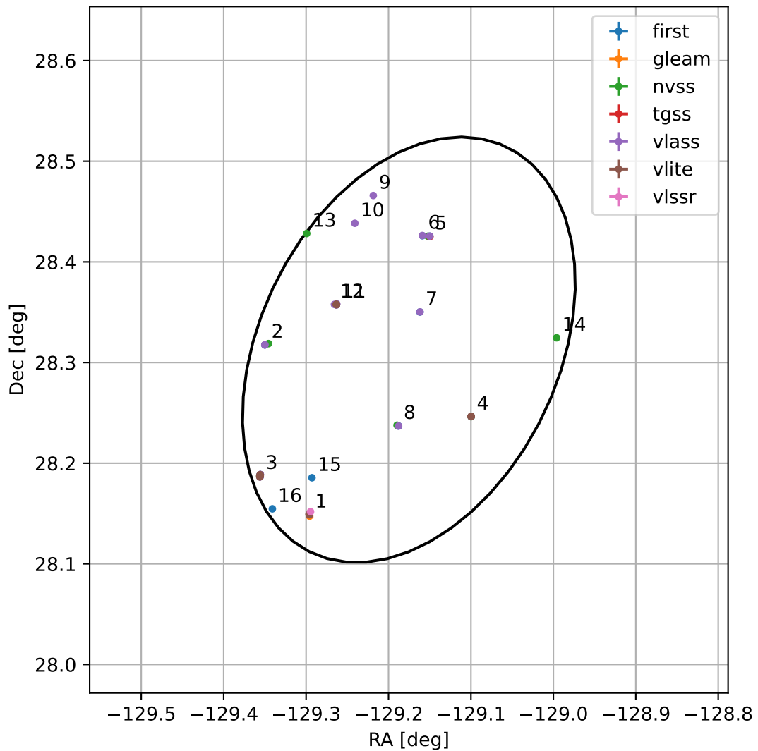
4FGL J1523.2+2818
