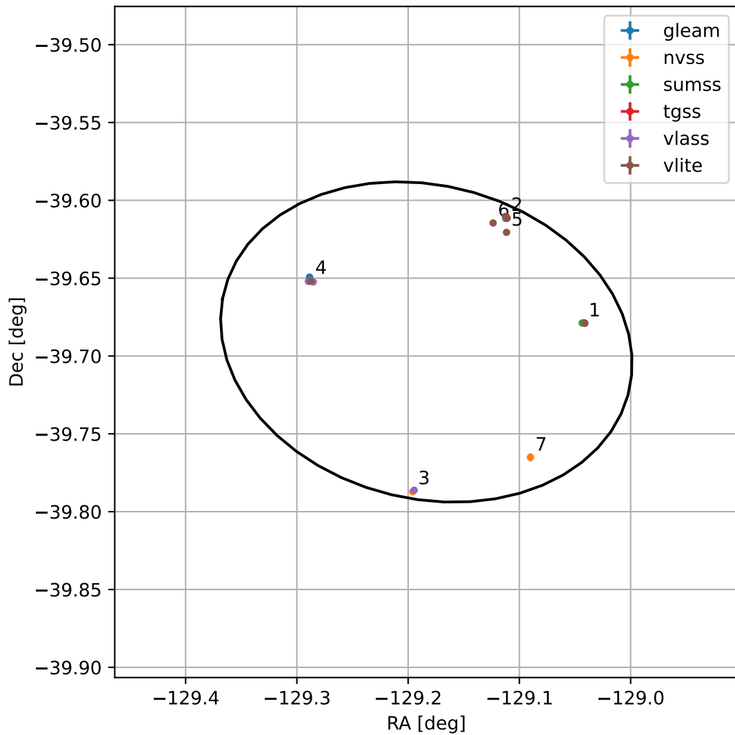
4FGL J1523.2-3941
