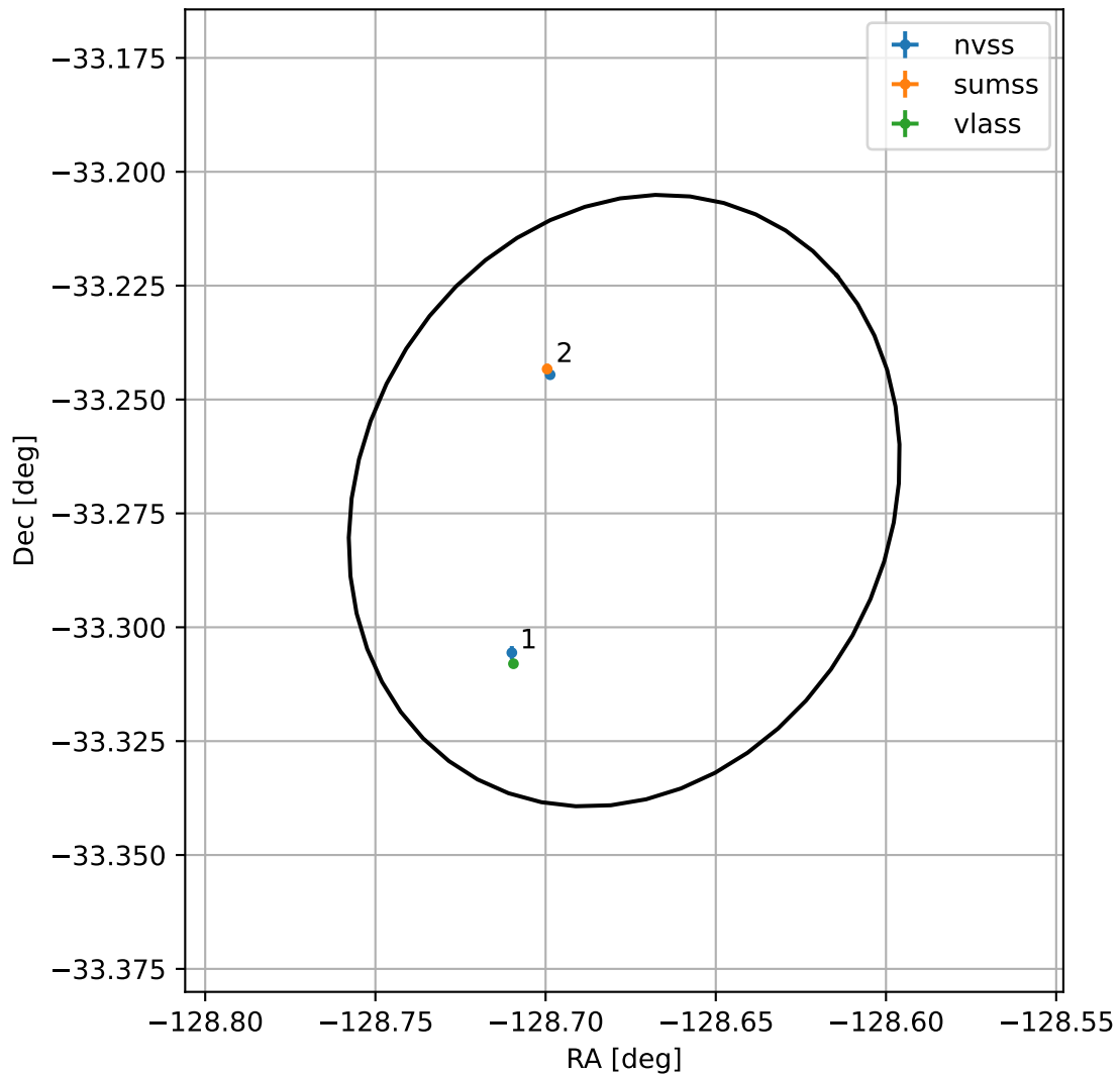
4FGL J1525.2-3316
