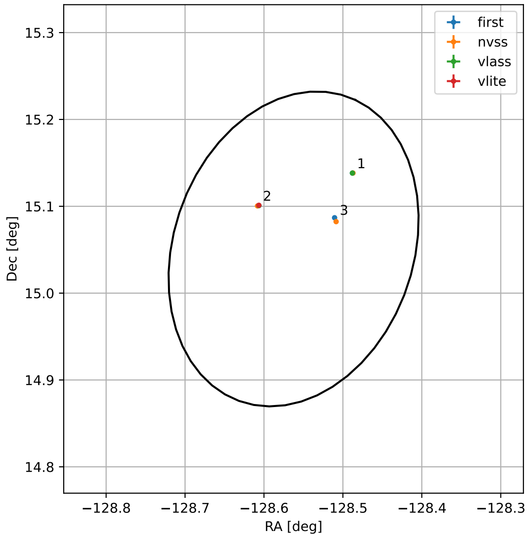
4FGL J1525.7+1503
