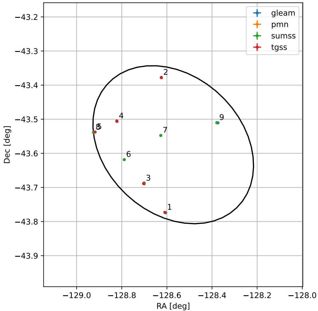
4FGL J1525.7-4334
