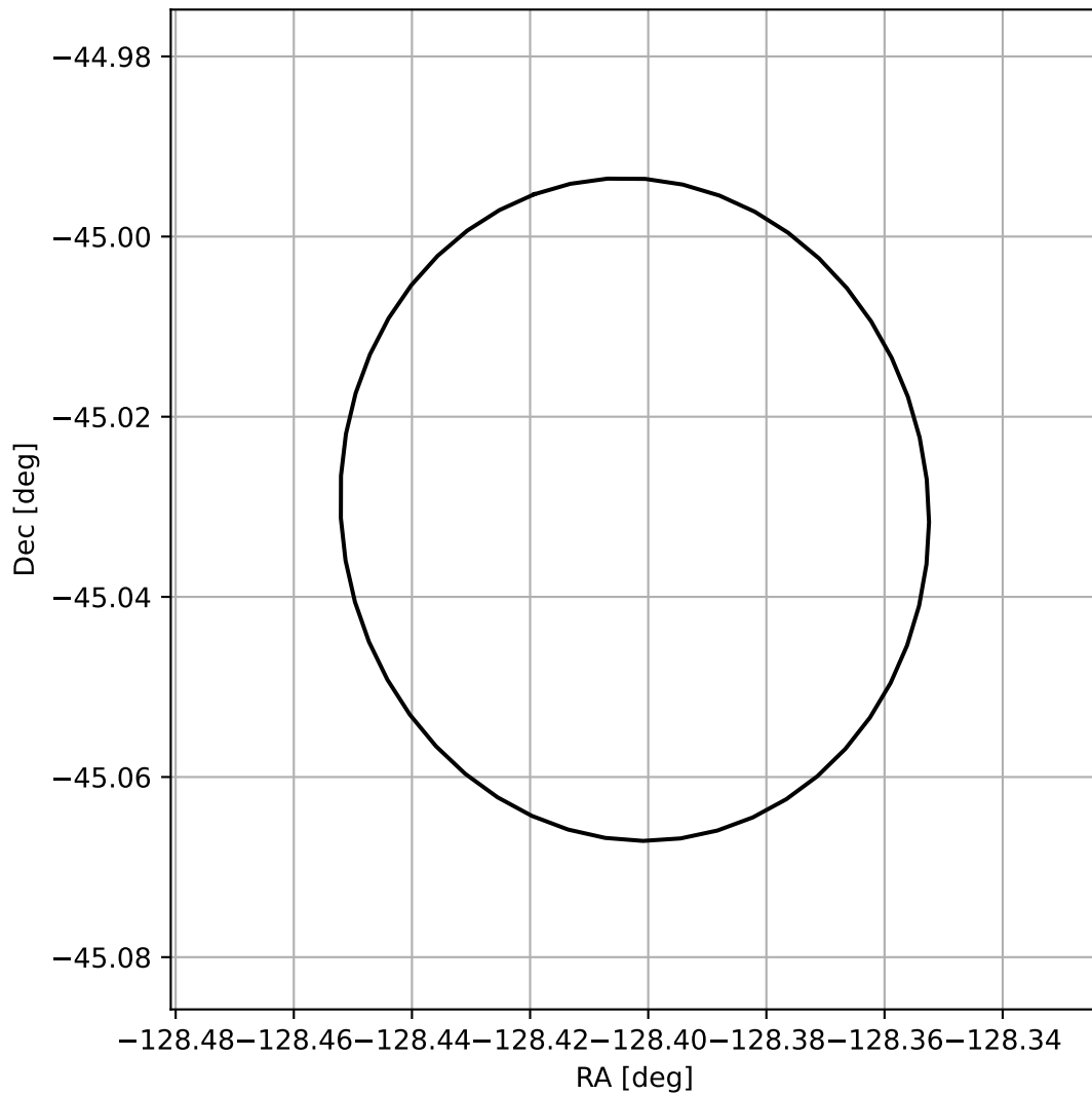
4FGL J1526.3-4501
