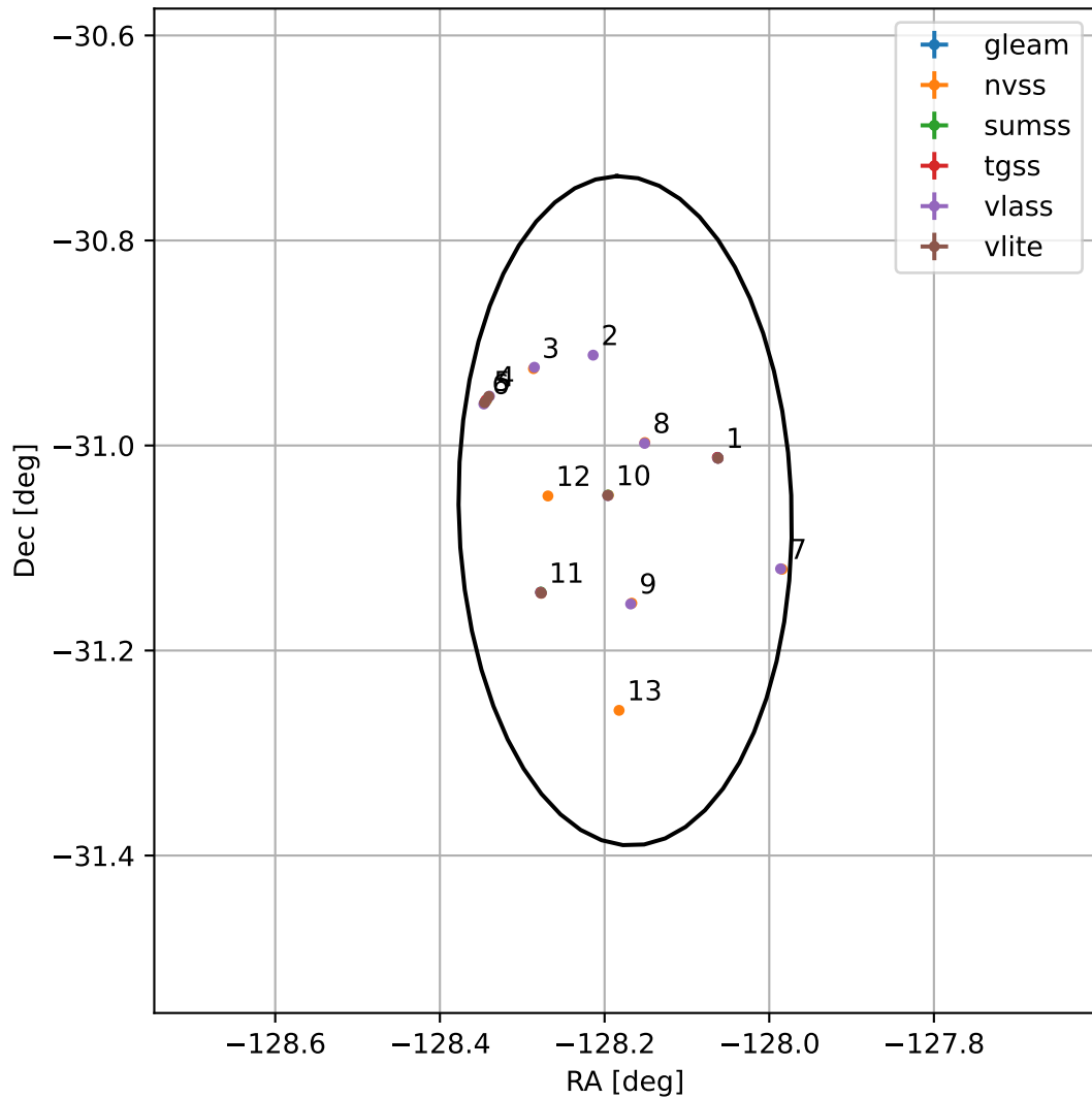
4FGL J1527.3-3103
