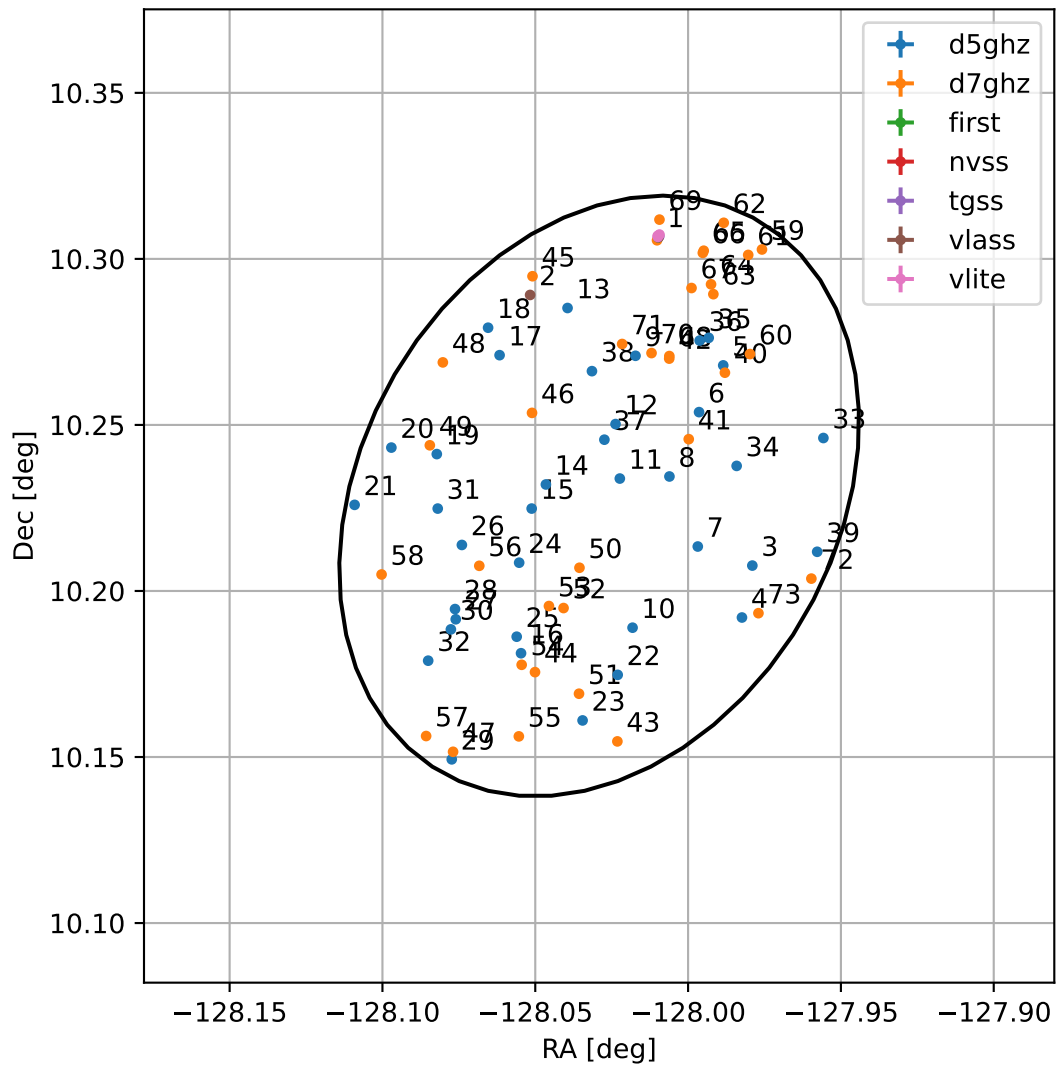
4FGL J1527.8+1013
