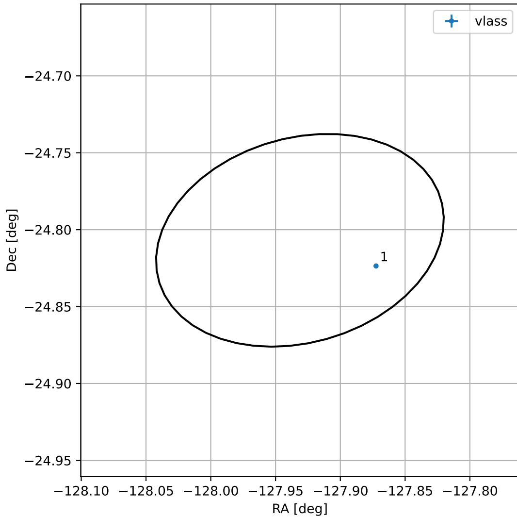
4FGL J1528.2-2448
