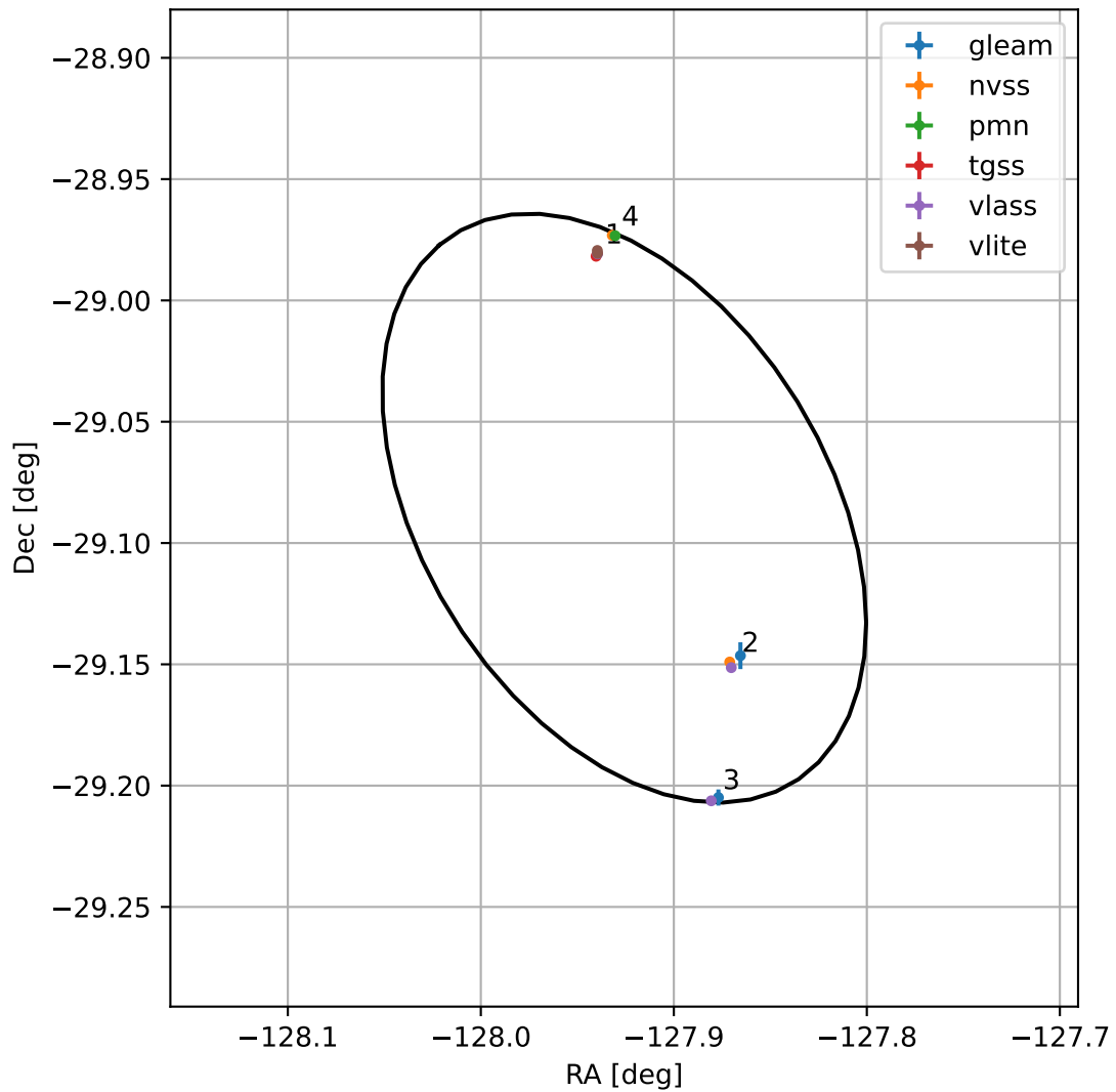
4FGL J1528.2-2905
