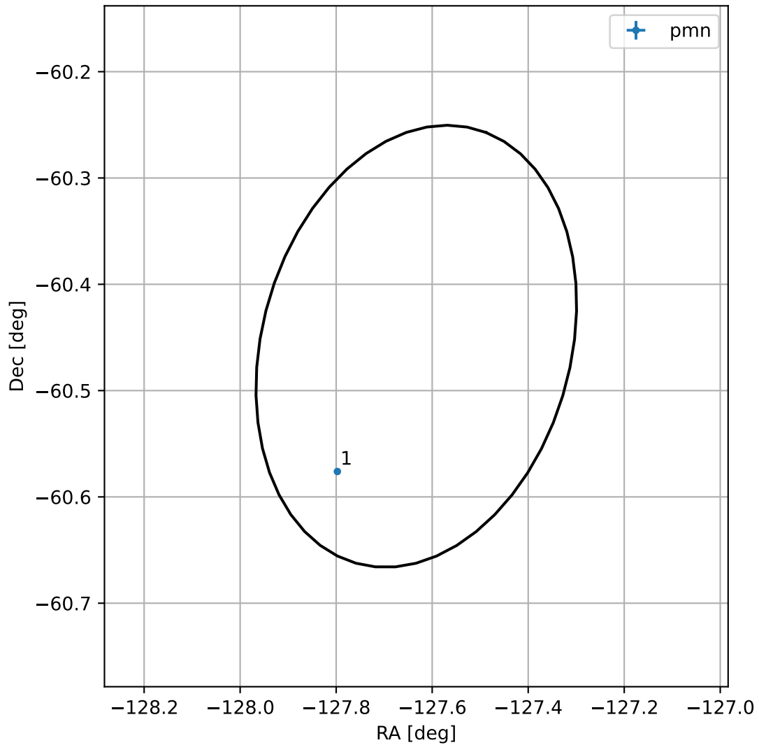
4FGL J1529.4-6027
