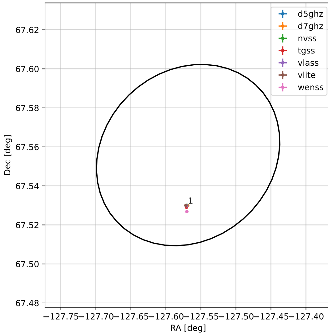
4FGL J1529.7+6733
