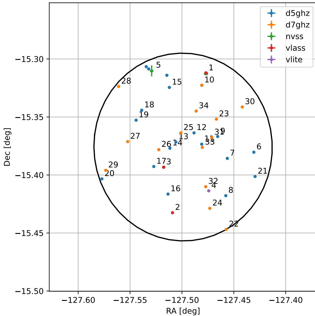
4FGL J1530.0-1522
