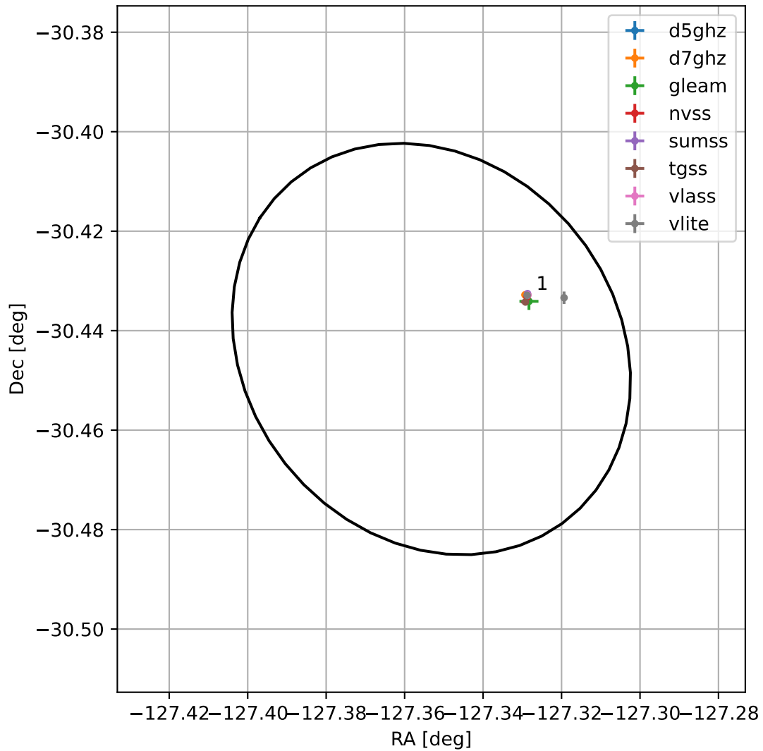
4FGL J1530.5-3026
