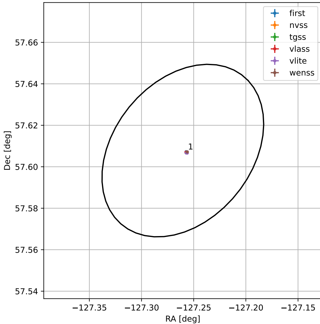
4FGL J1530.9+5736
