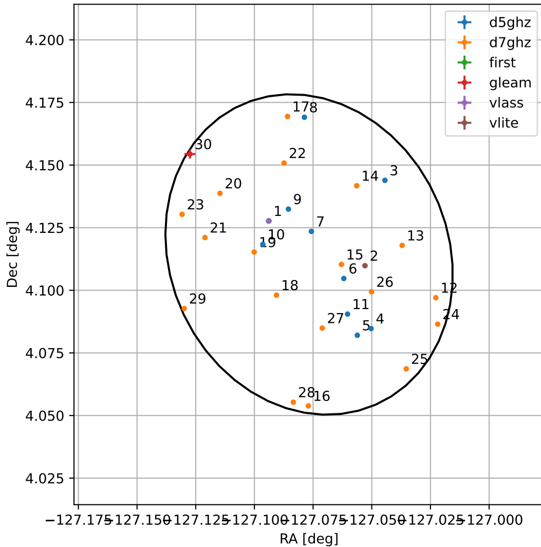
4FGL J1531.6+0406
