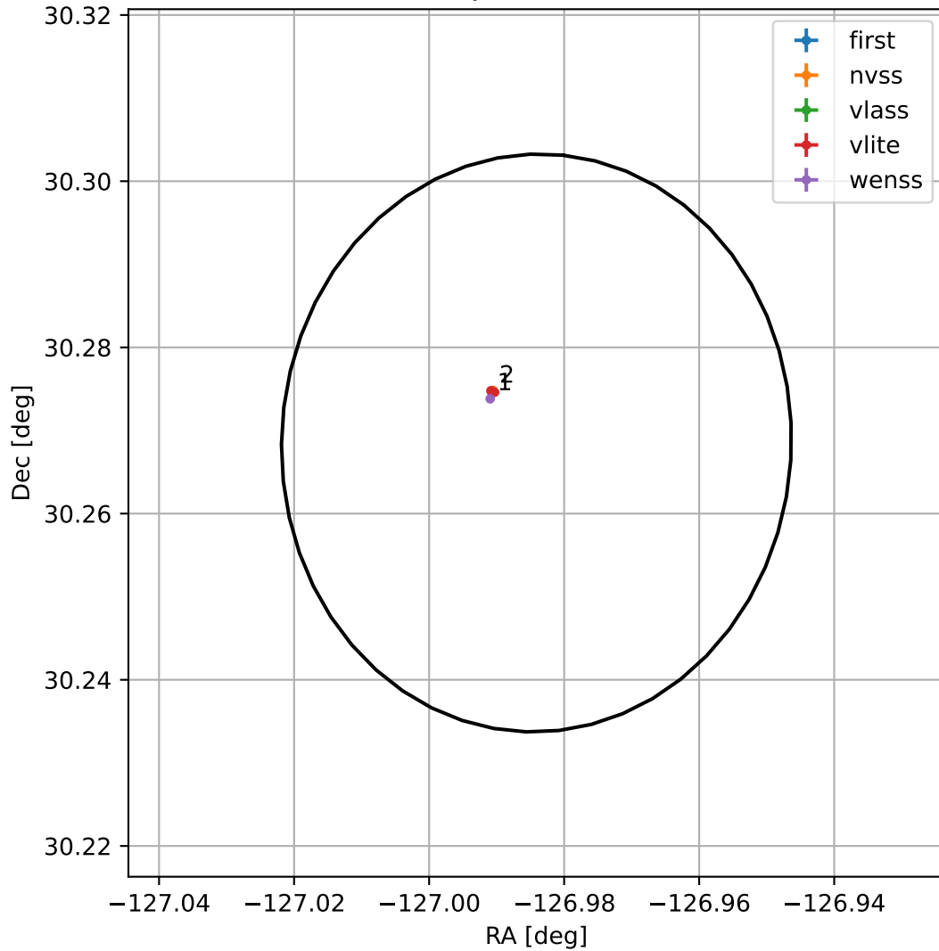
4FGL J1532.0+3016
