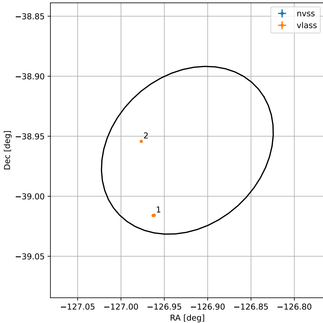
4FGL J1532.3-3857
