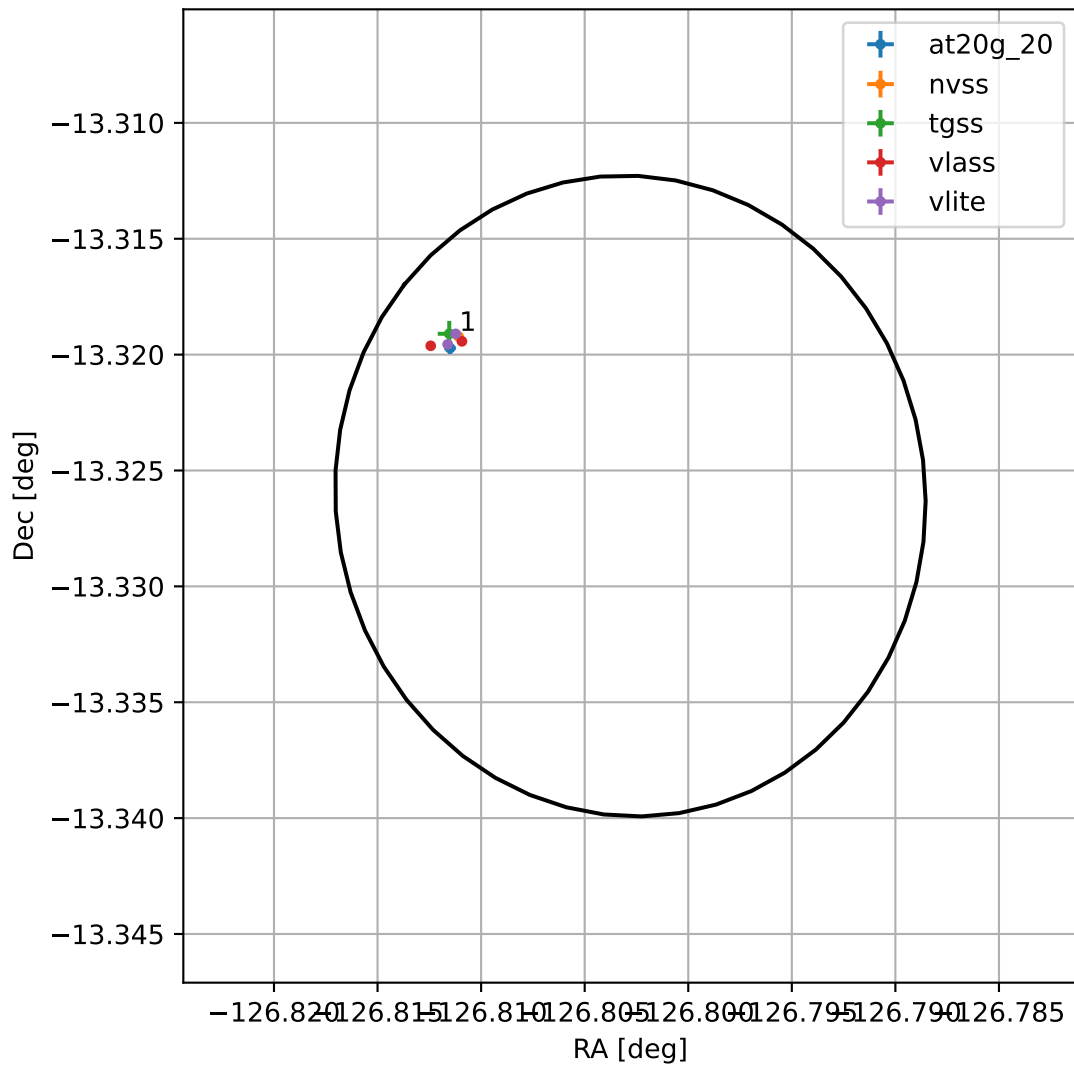
4FGL J1532.7-1319
