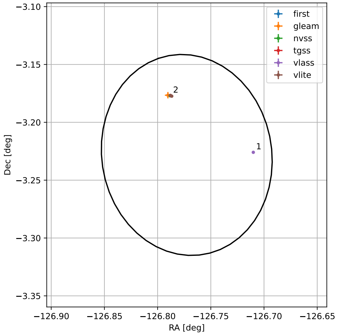
4FGL J1532.9-0313
