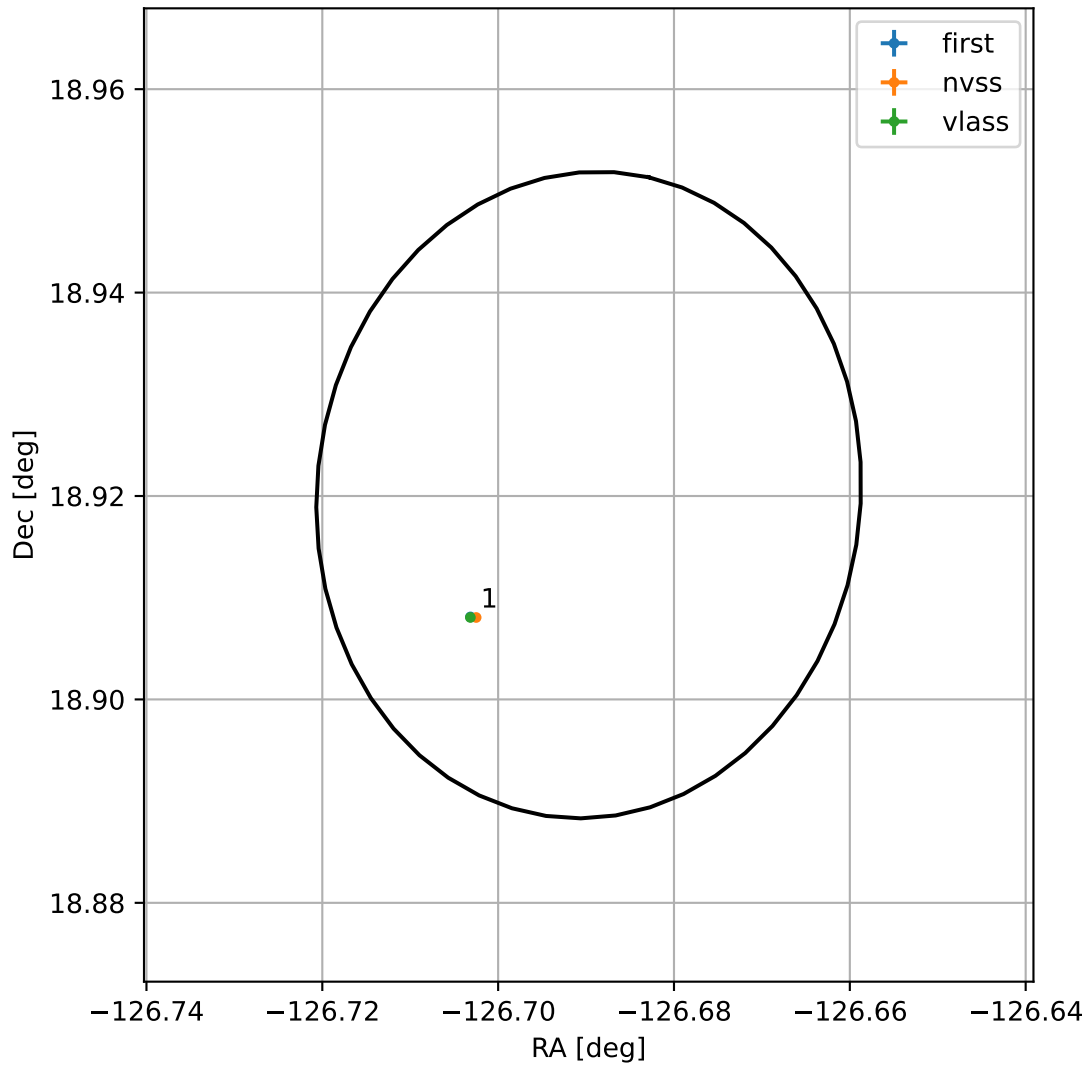
4FGL J1533.2+1855
