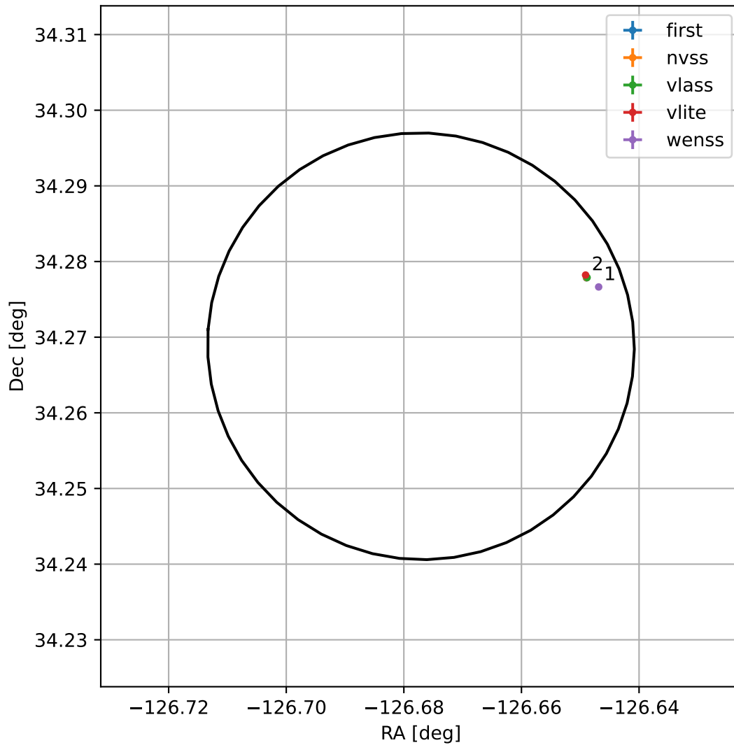
4FGL J1533.2+3416
