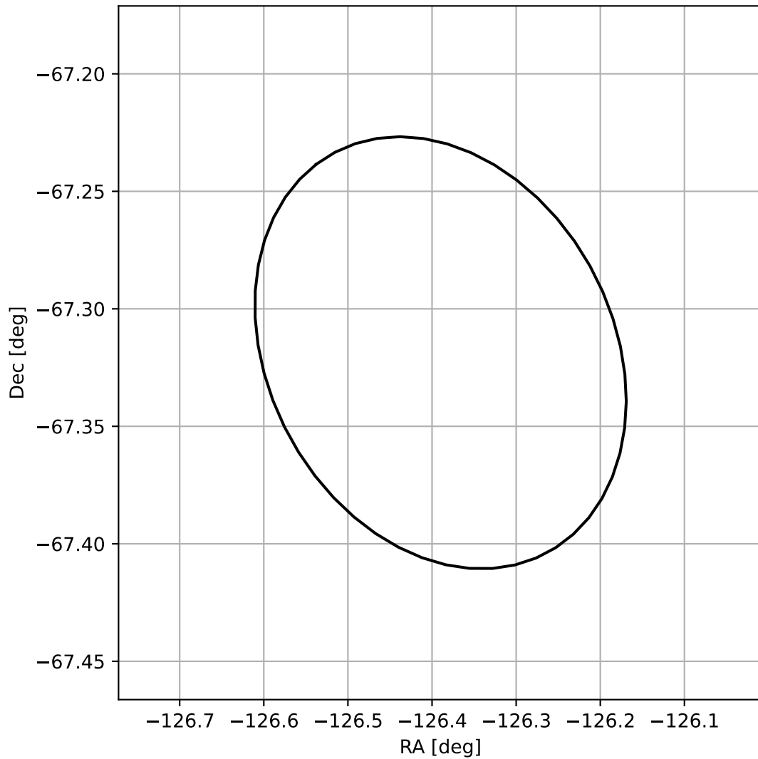
4FGL J1534.4-6719
