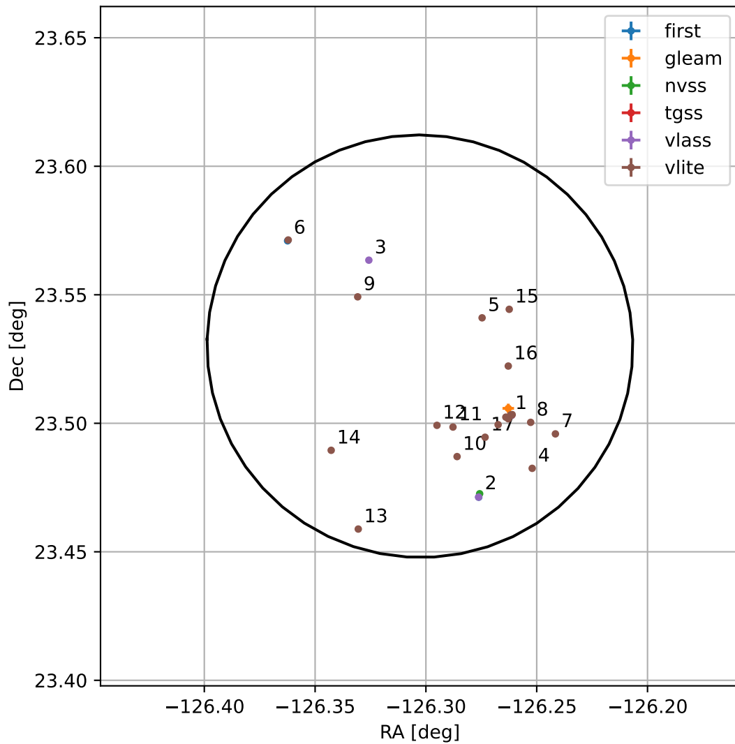
4FGL J1534.7+2331
