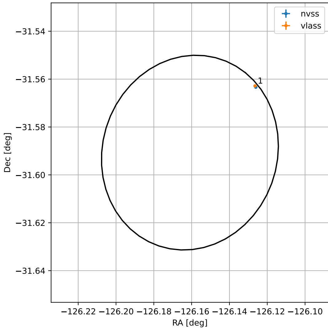
4FGL J1535.3-3135
