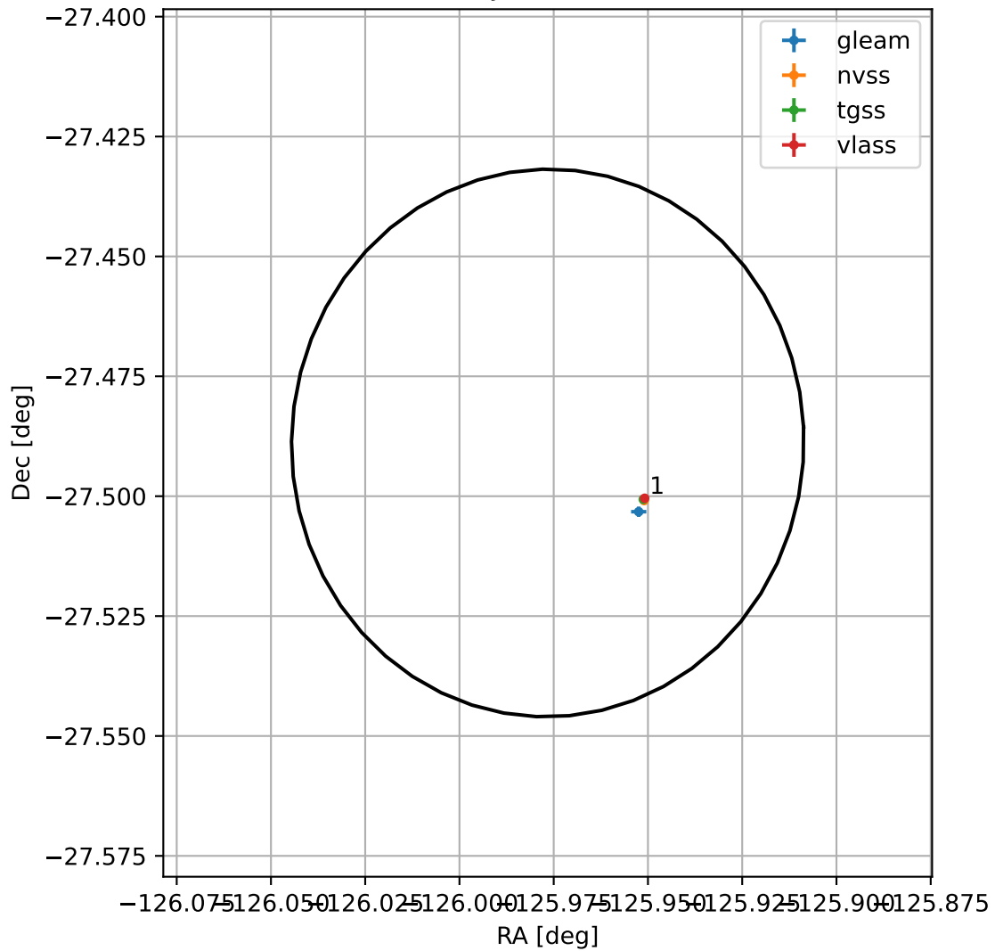
4FGL J1536.0-2729
