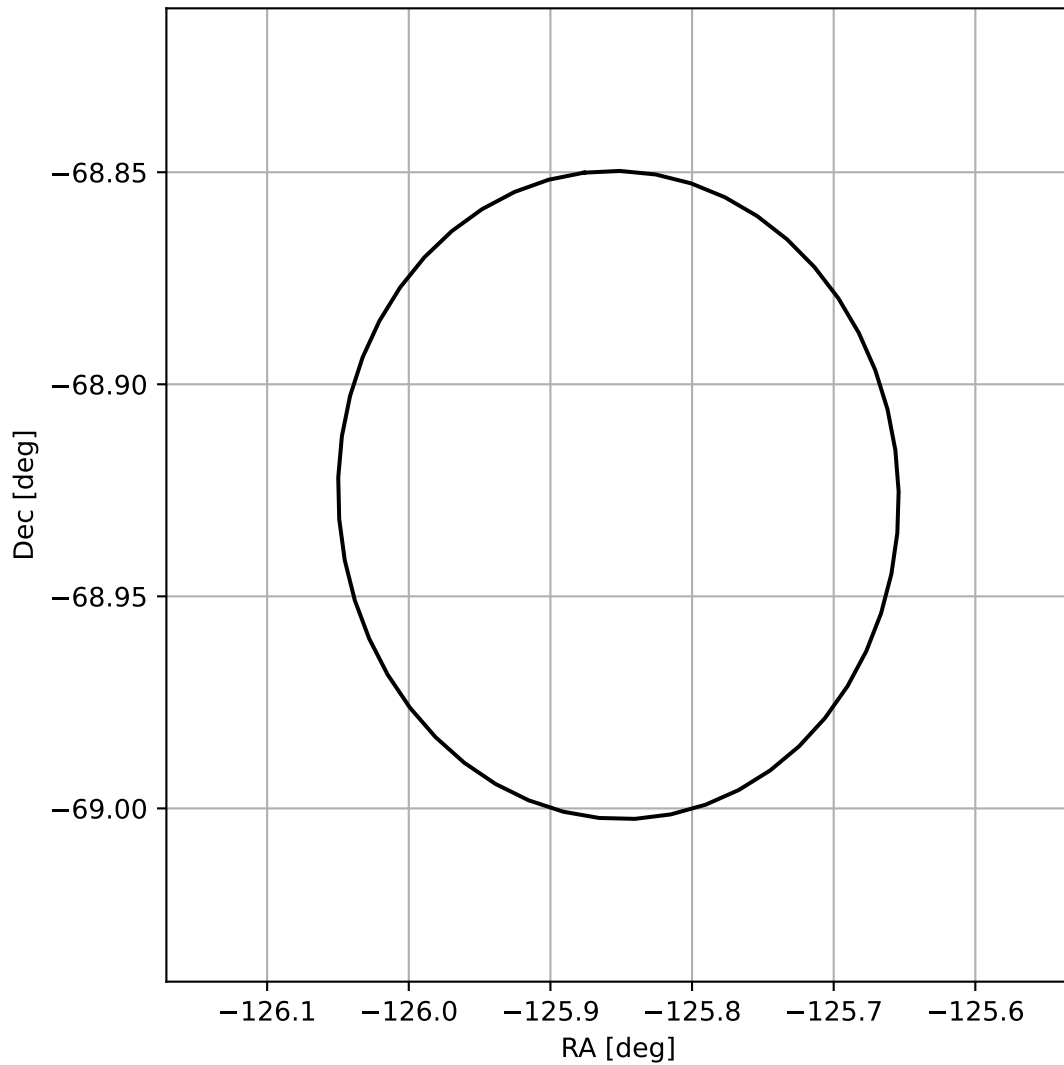
4FGL J1536.5-6855
