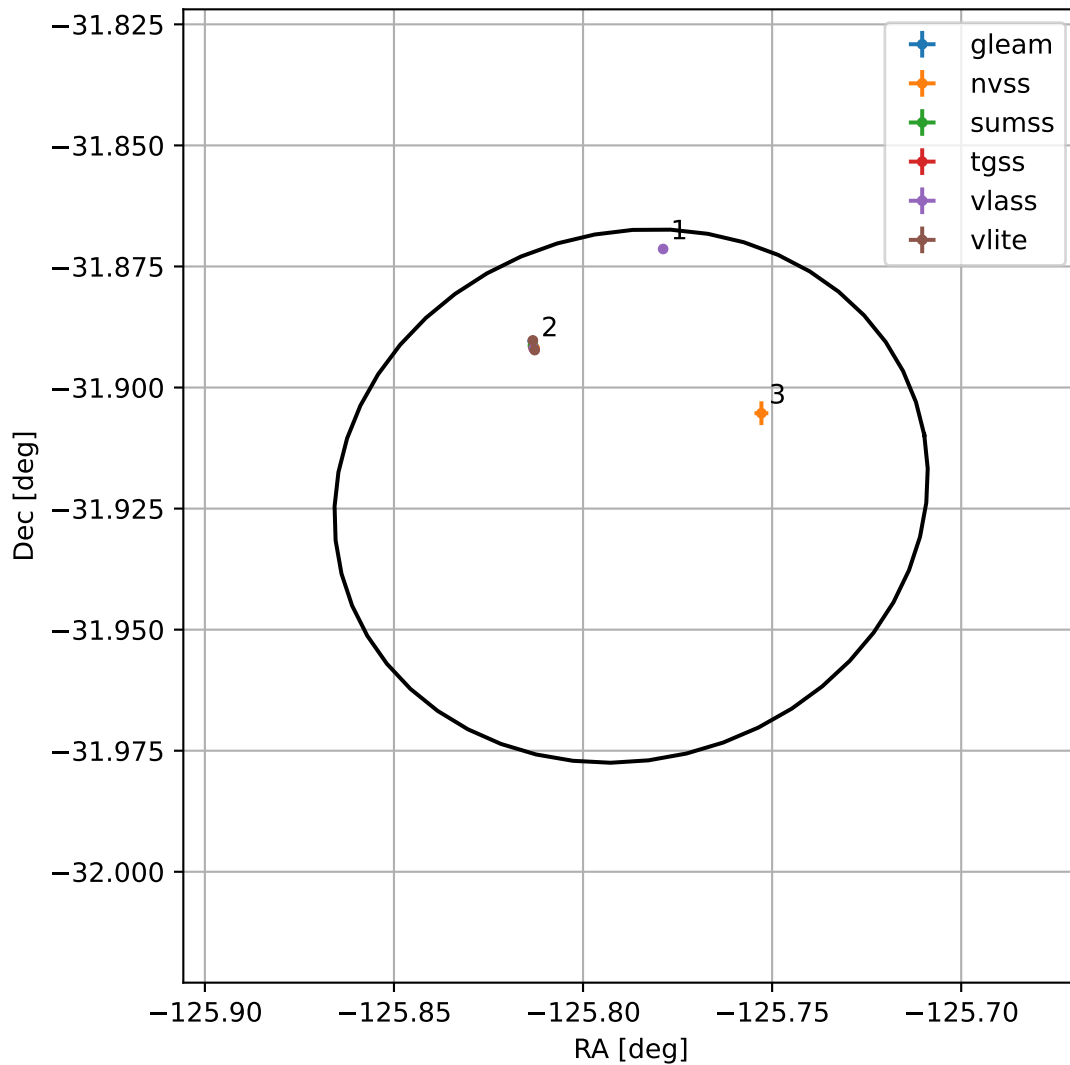
4FGL J1536.8-3155
