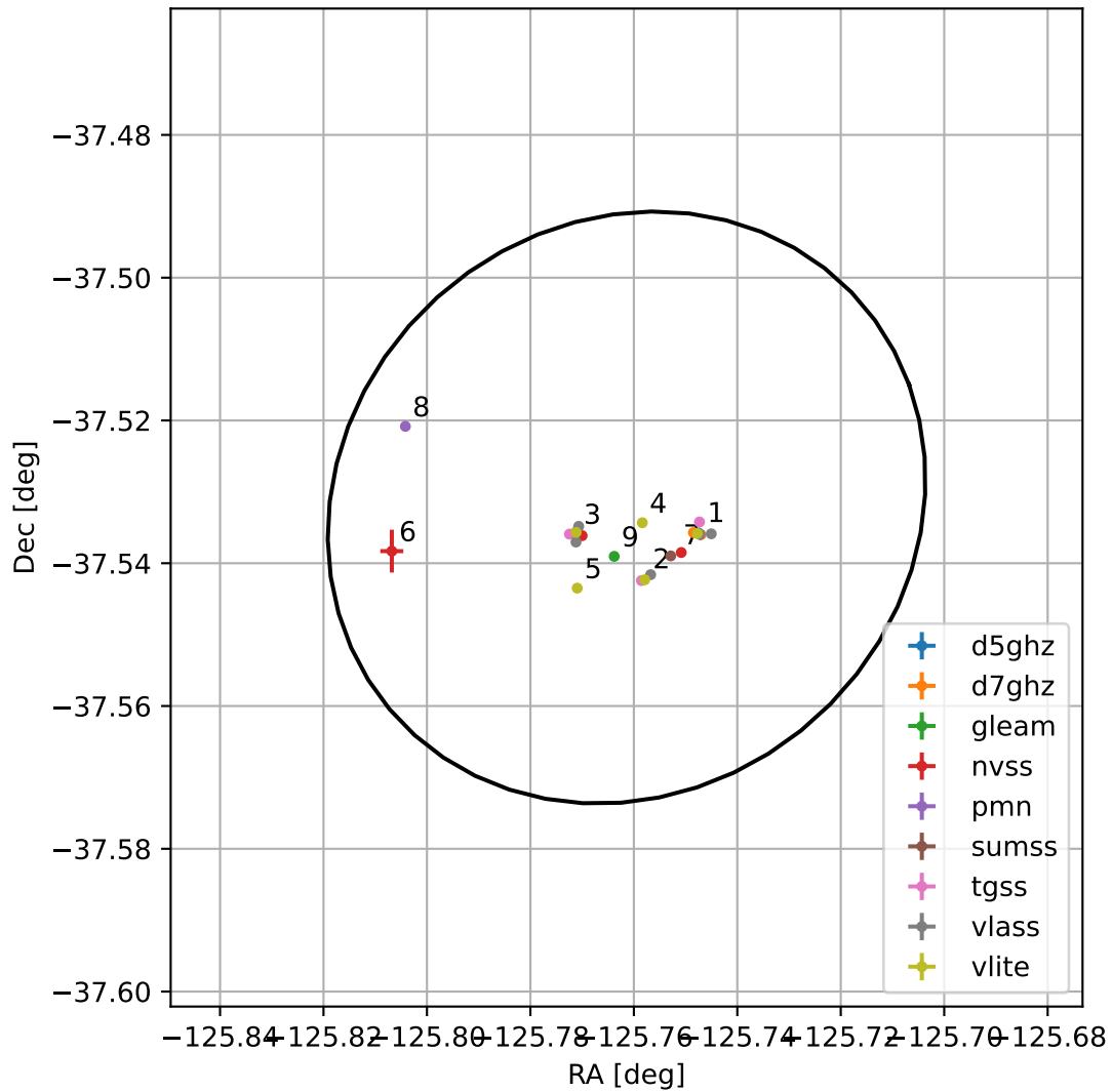
4FGL J1536.9-3731
