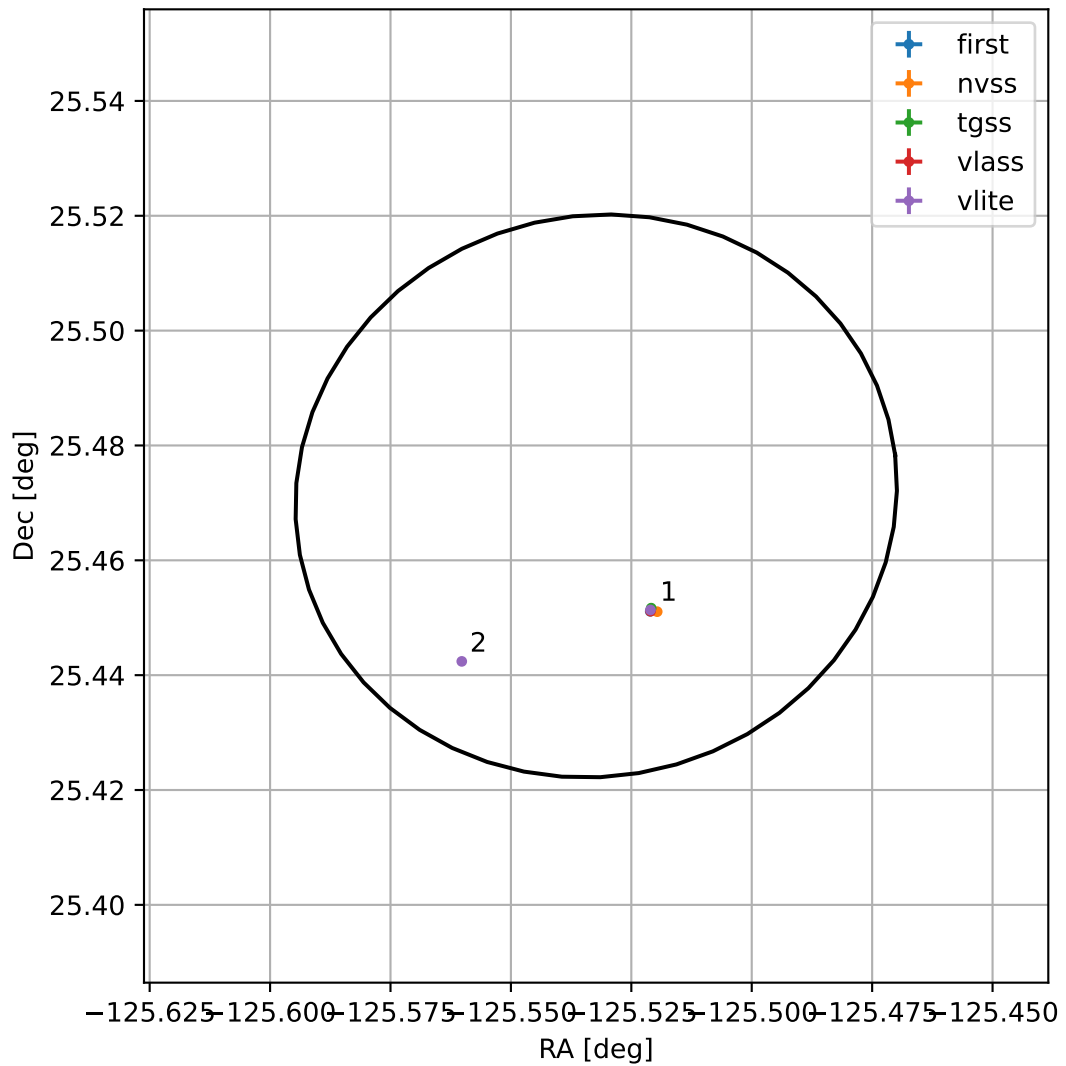
4FGL J1537.8+2528
