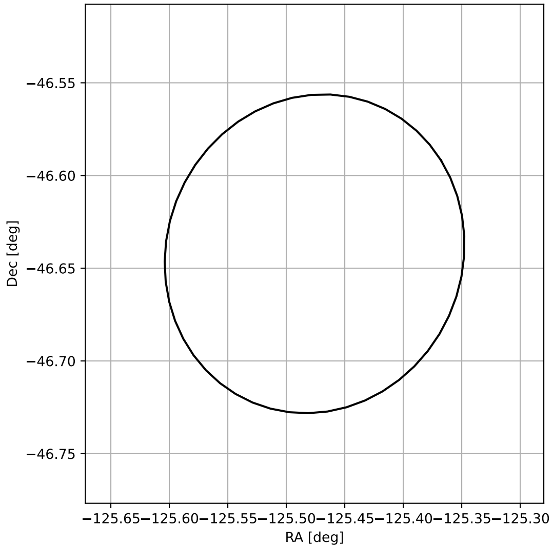
4FGL J1538.0-4638
