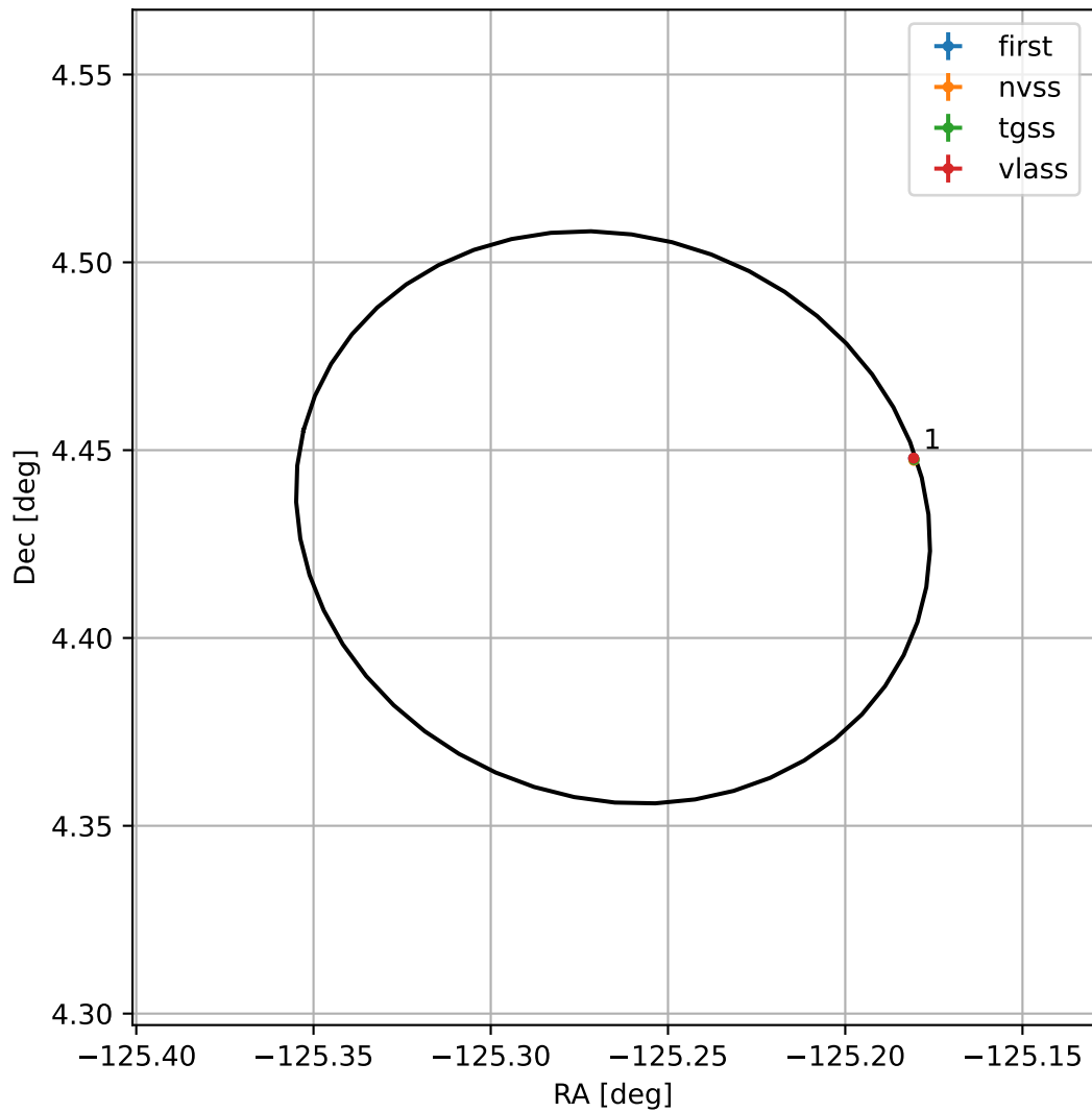
4FGL J1538.9+0425
