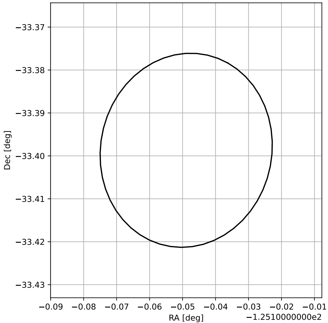
4FGL J1539.4-3323
