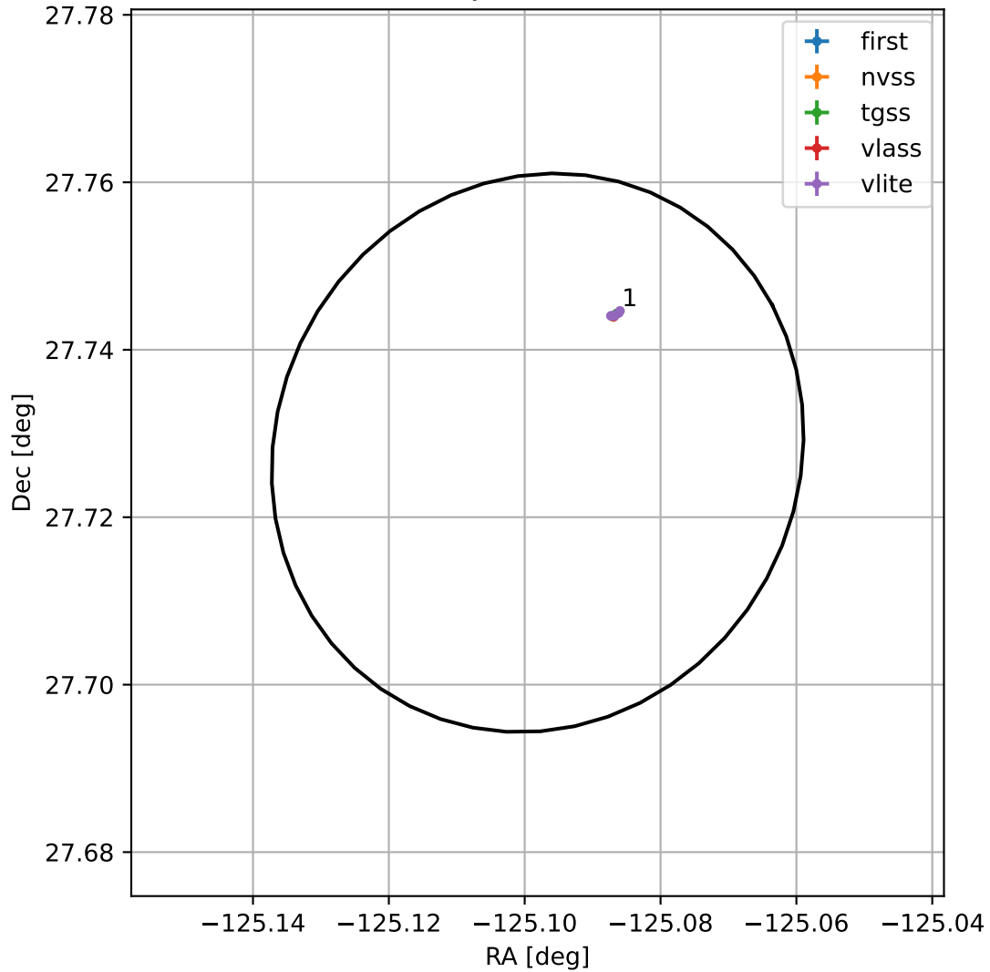
4FGL J1539.6+2743
