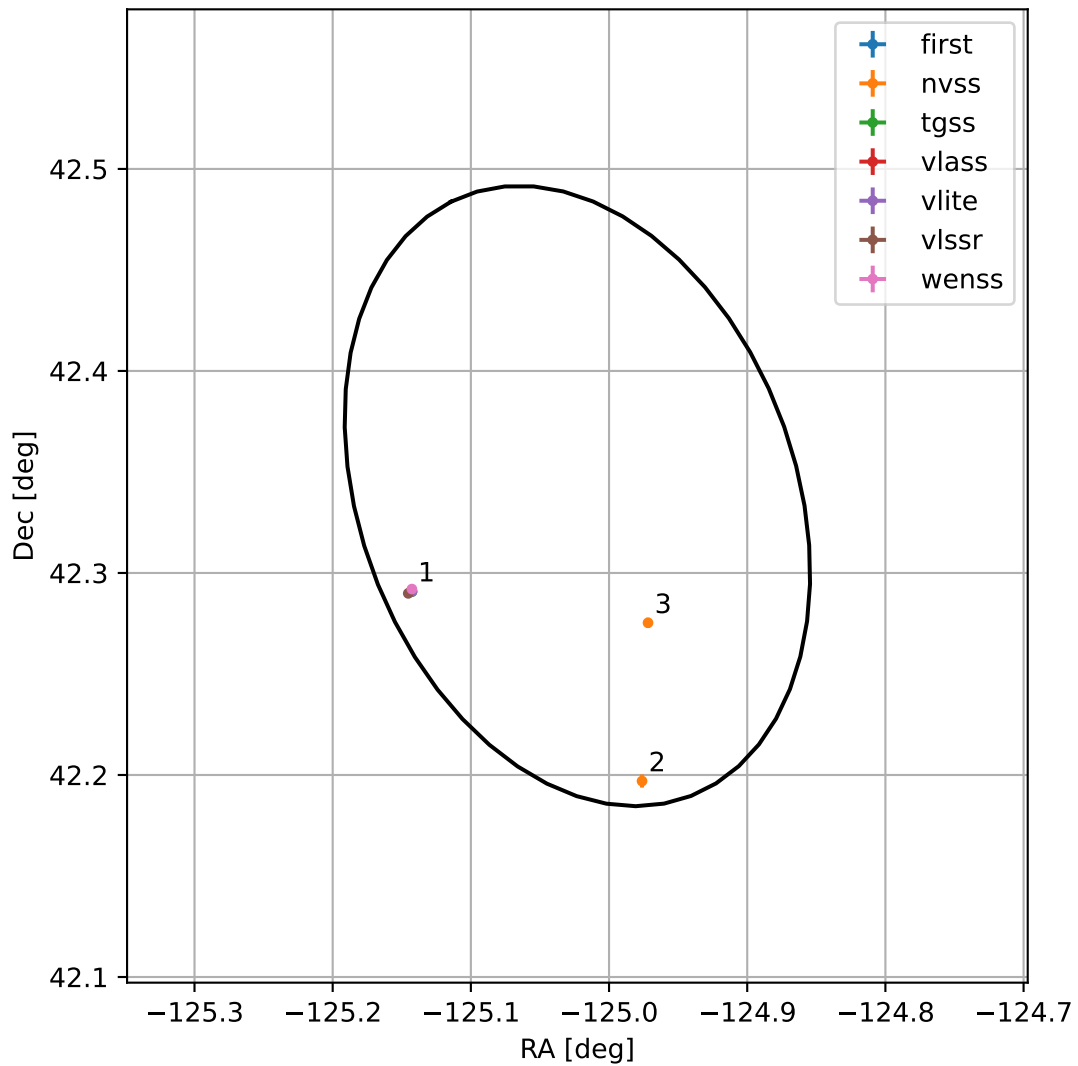
4FGL J1539.9+4220
