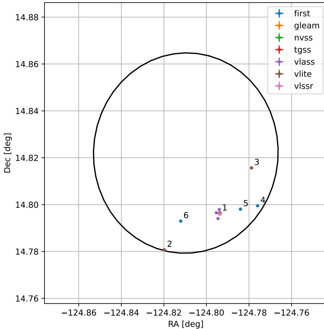
4FGL J1540.7+1449
