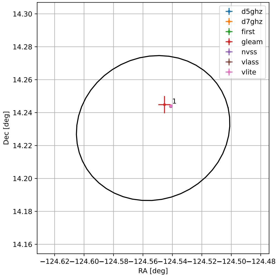
4FGL J1541.7+1413
