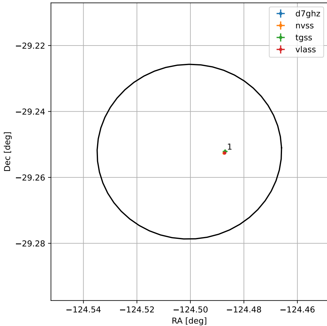
4FGL J1541.9-2915
