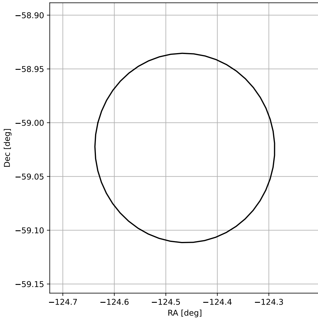
4FGL J1542.1-5901
