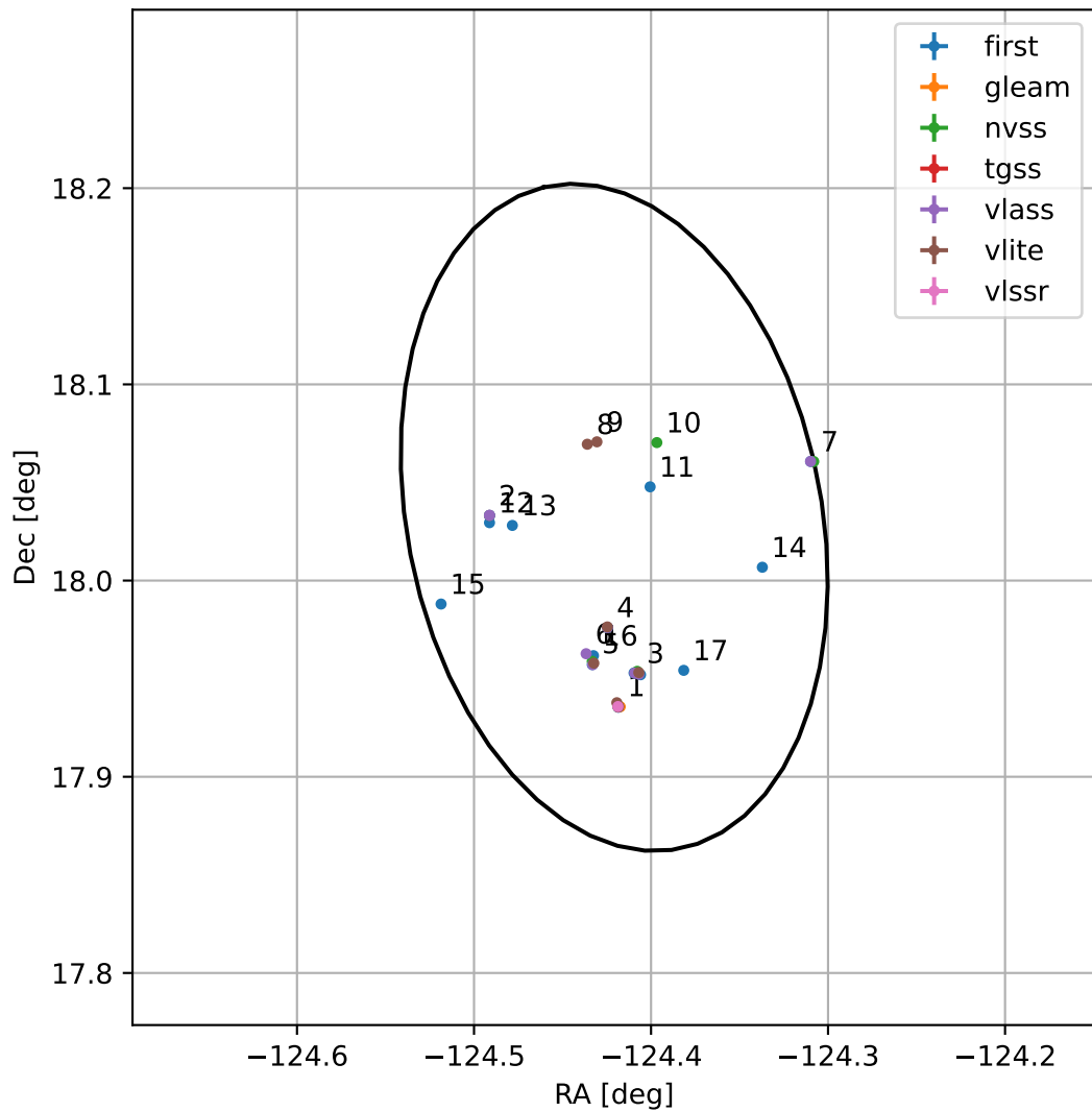
4FGL J1542.3+1801
